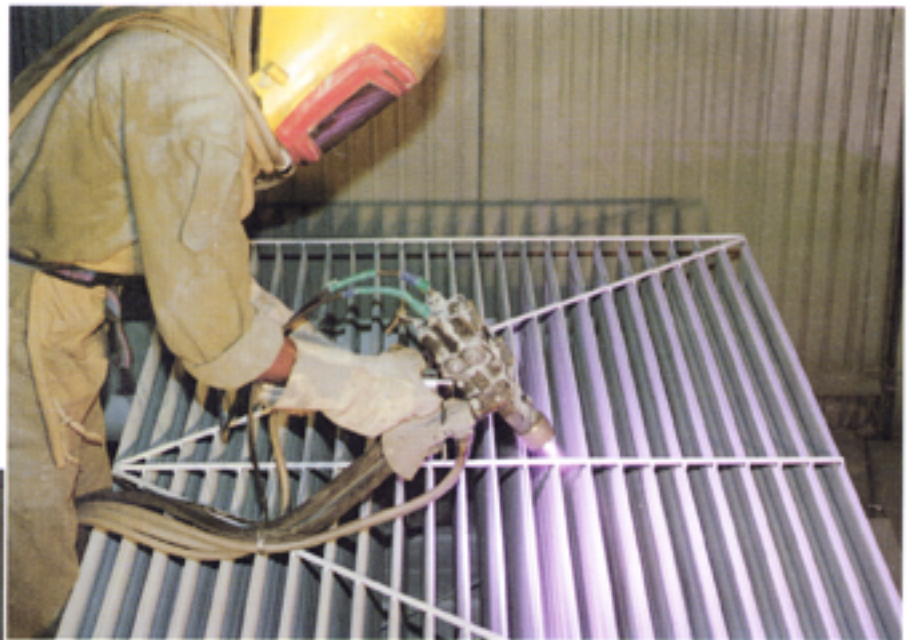
Arc Spray Galvanizing
